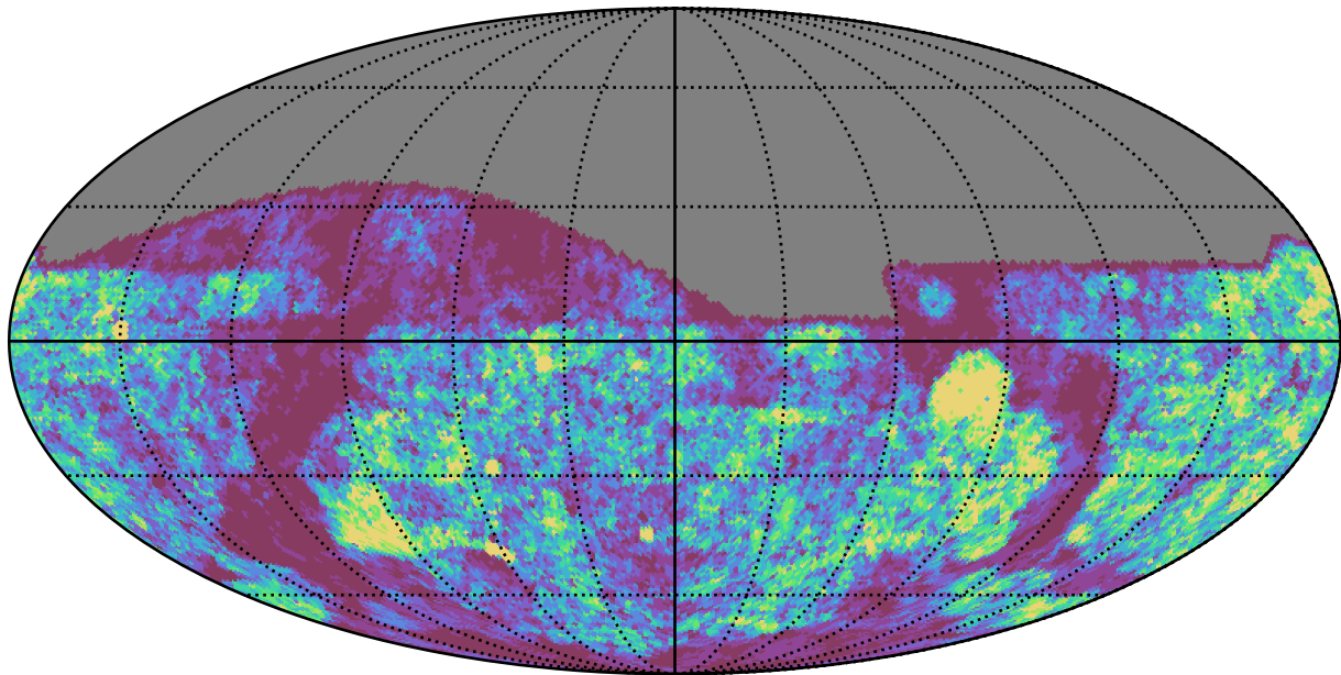
baseline_v3.4_10yrs g band: Gaps_24hr
