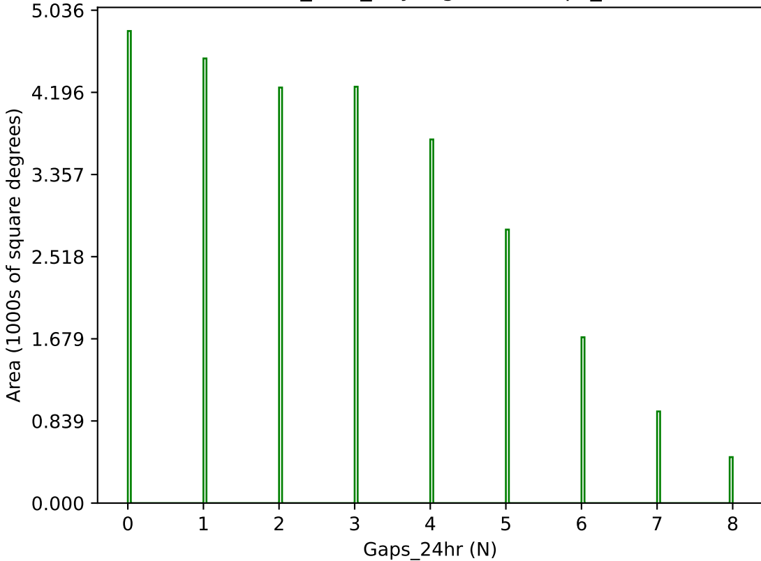
baseline_v3.4_10yrs g band: Gaps_24hr
