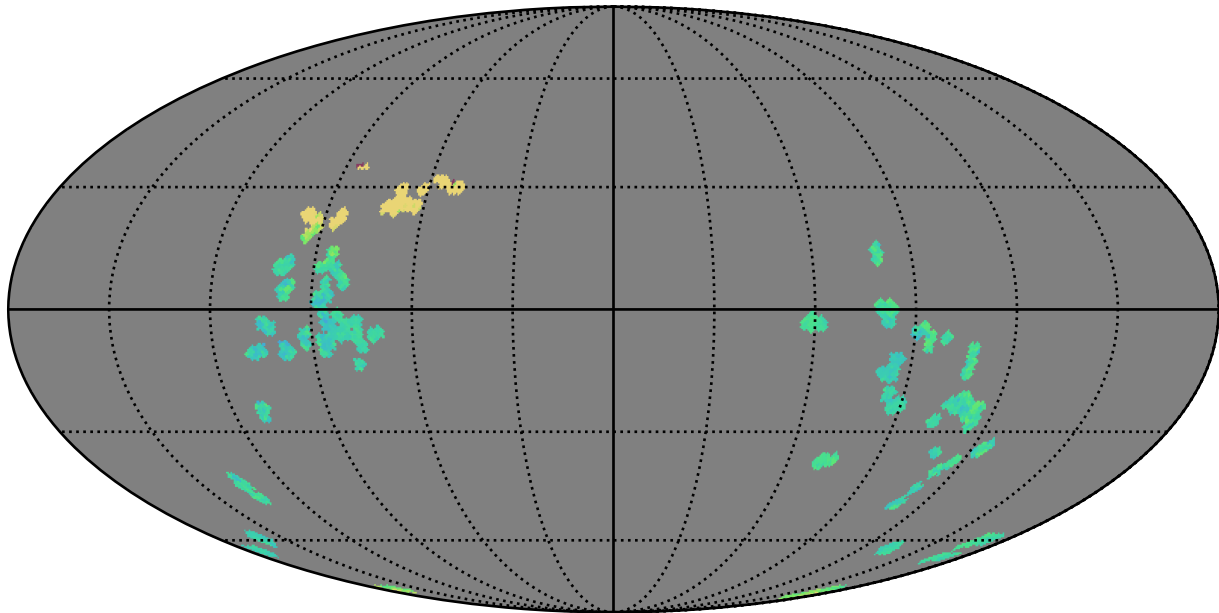
baseline_v3.4_10yrs : GalplaneTimePerFilter_zucker_sfr_map_z
