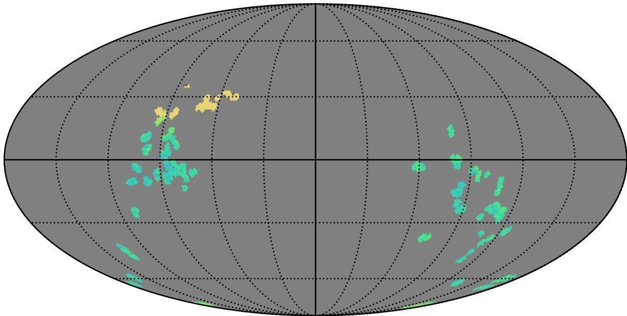
baseline_v3.4_10yrs : GalplaneTimePerFilter_zucker_sfr_map_z
