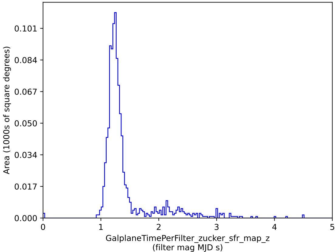
baseline_v3.4_10yrs : GalplaneTimePerFilter_zucker_sfr_map_z
