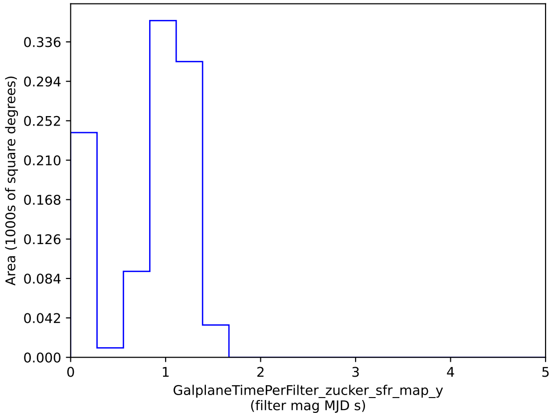
baseline_v3.4_10yrs : GalplaneTimePerFilter_zucker_sfr_map_y
