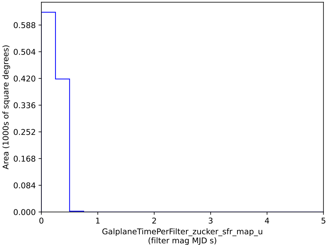
baseline_v3.4_10yrs : GalplaneTimePerFilter_zucker_sfr_map_u
