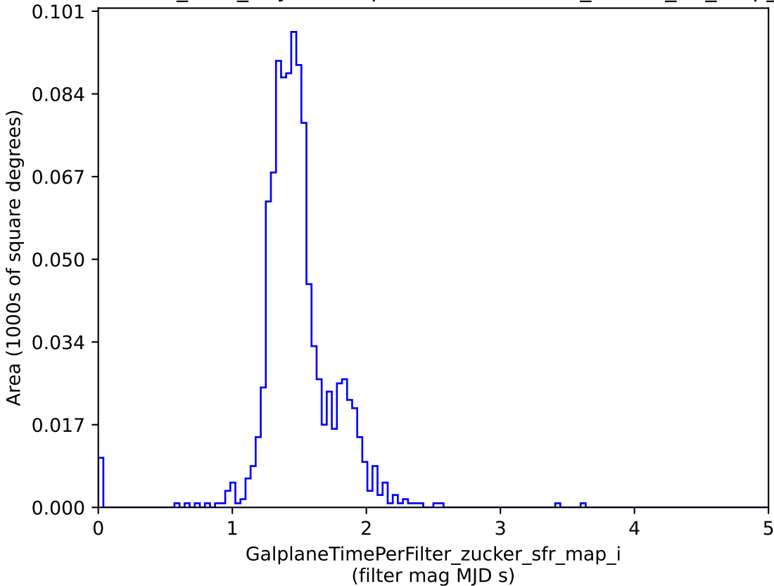
baseline_v3.4_10yrs : GalplaneTimePerFilter_zucker_sfr_map_i
