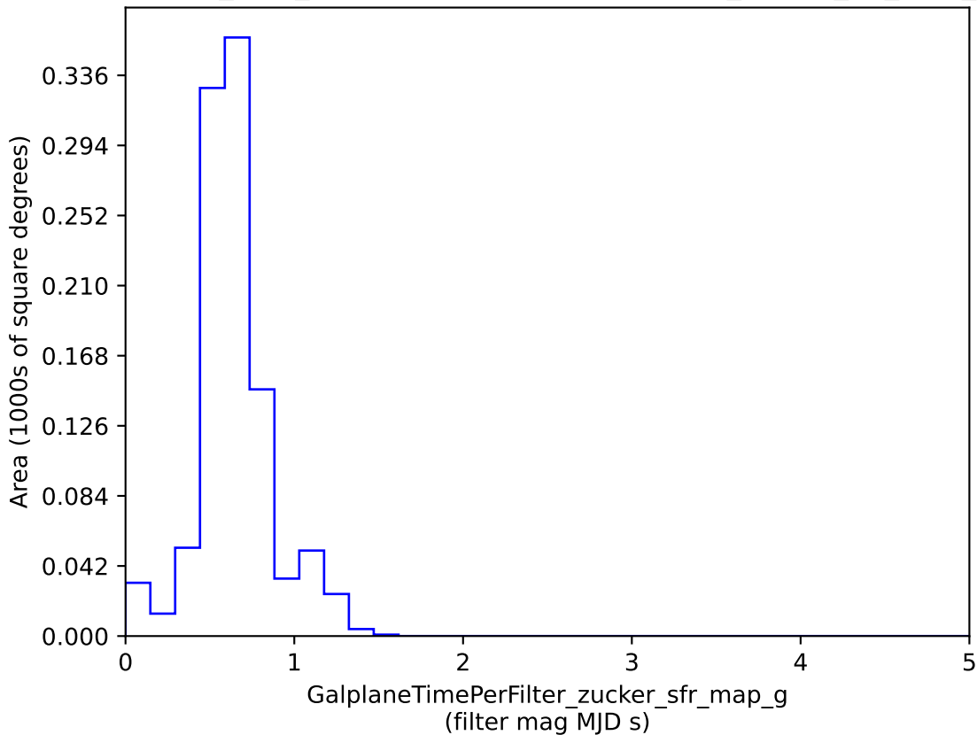
baseline_v3.4_10yrs : GalplaneTimePerFilter_zucker_sfr_map_g
