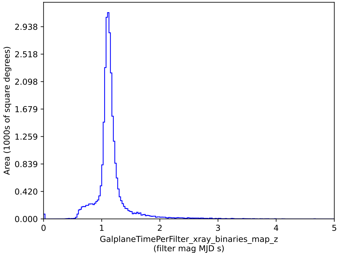
baseline_v3.4_10yrs : GalplaneTimePerFilter_xray_binaries_map_z
