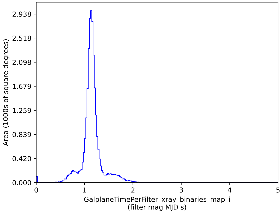
baseline_v3.4_10yrs : GalplaneTimePerFilter_xray_binaries_map_i
