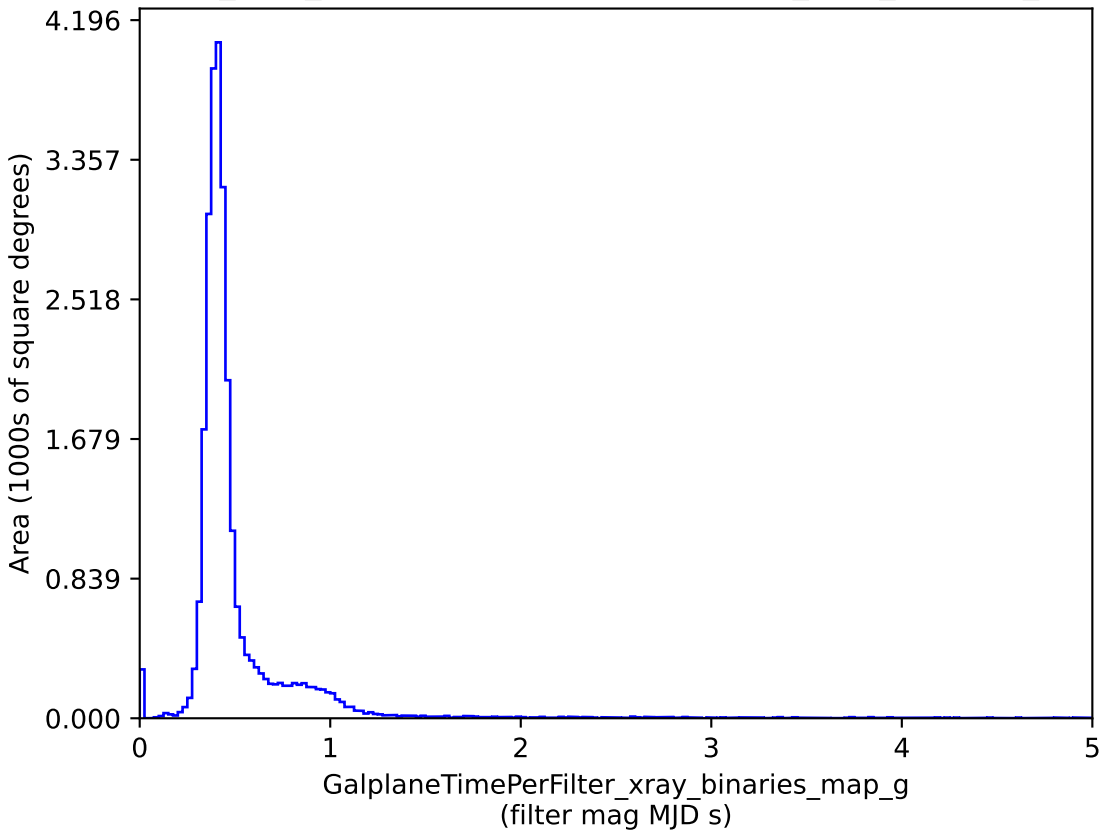
baseline_v3.4_10yrs : GalplaneTimePerFilter_xray_binaries_map_g
