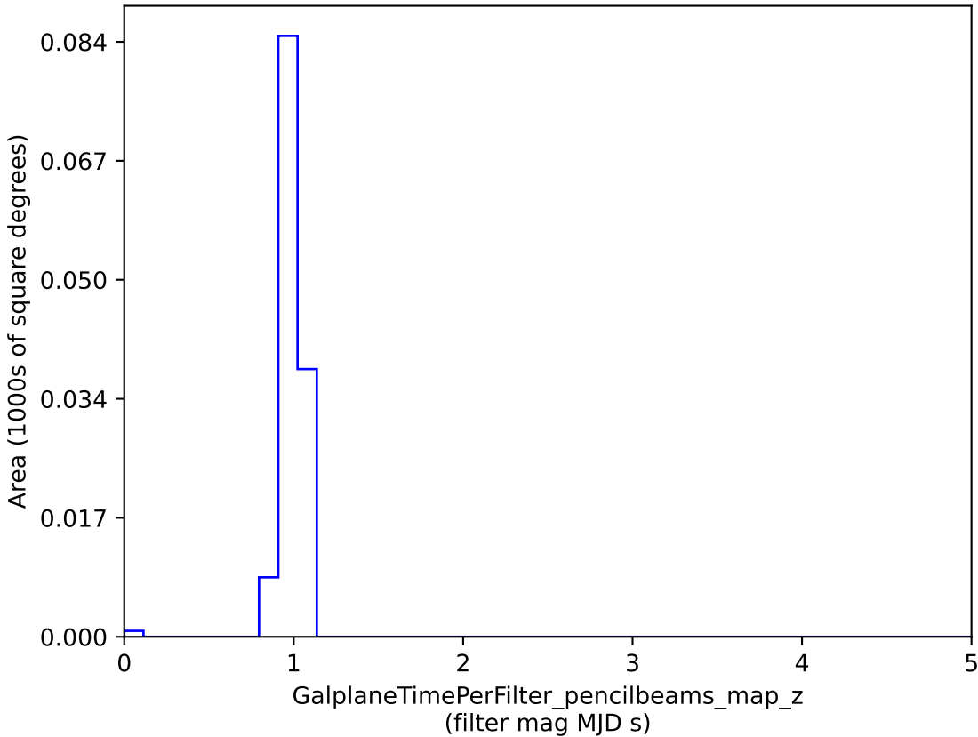
baseline_v3.4_10yrs : GalplaneTimePerFilter_pencilbeams_map_z
