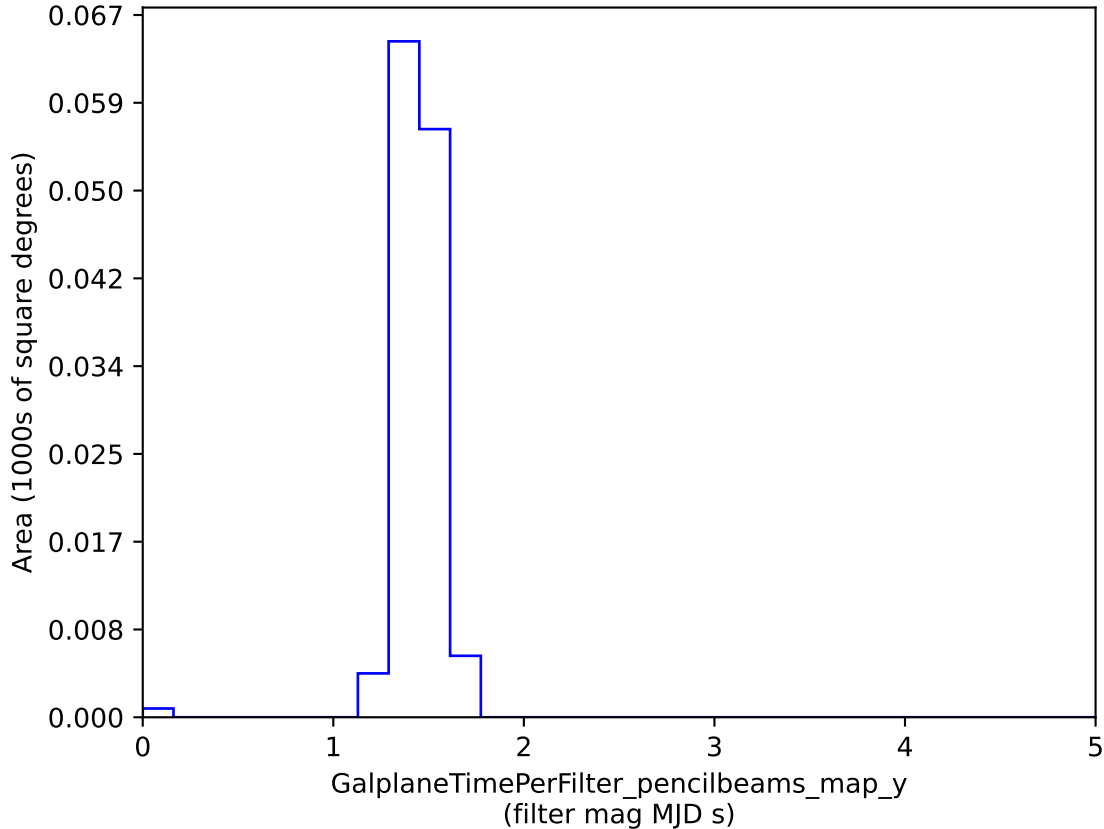
baseline_v3.4_10yrs : GalplaneTimePerFilter_pencilbeams_map_y
