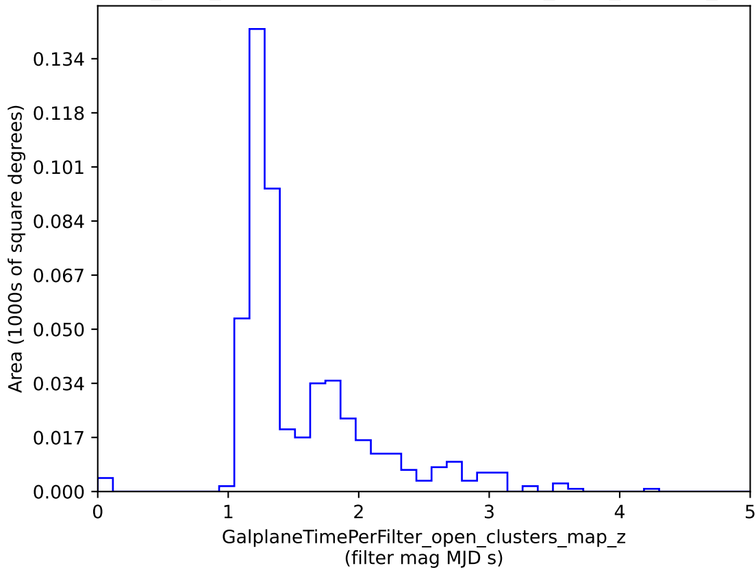
baseline_v3.4_10yrs : GalplaneTimePerFilter_open_clusters_map_z
