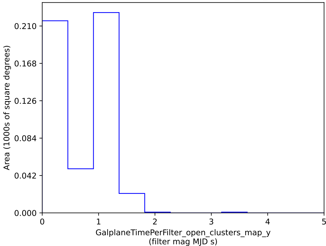
baseline_v3.4_10yrs : GalplaneTimePerFilter_open_clusters_map_y
