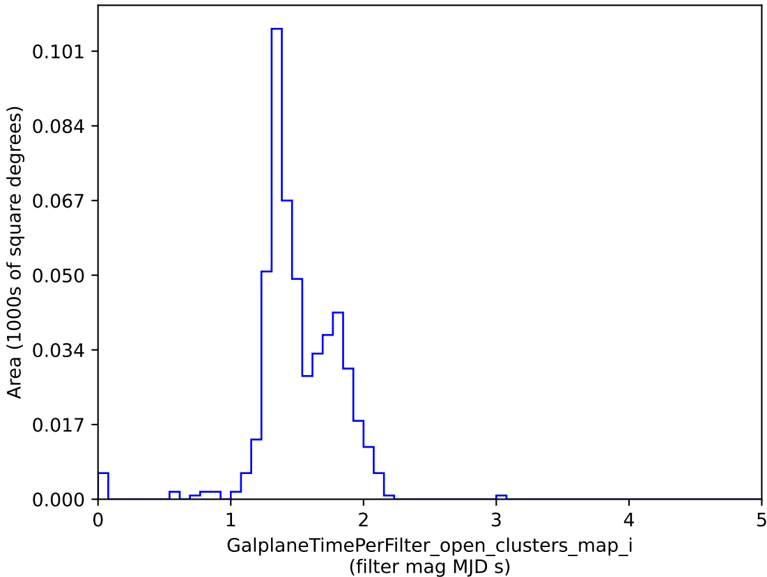
baseline_v3.4_10yrs : GalplaneTimePerFilter_open_clusters_map_i
