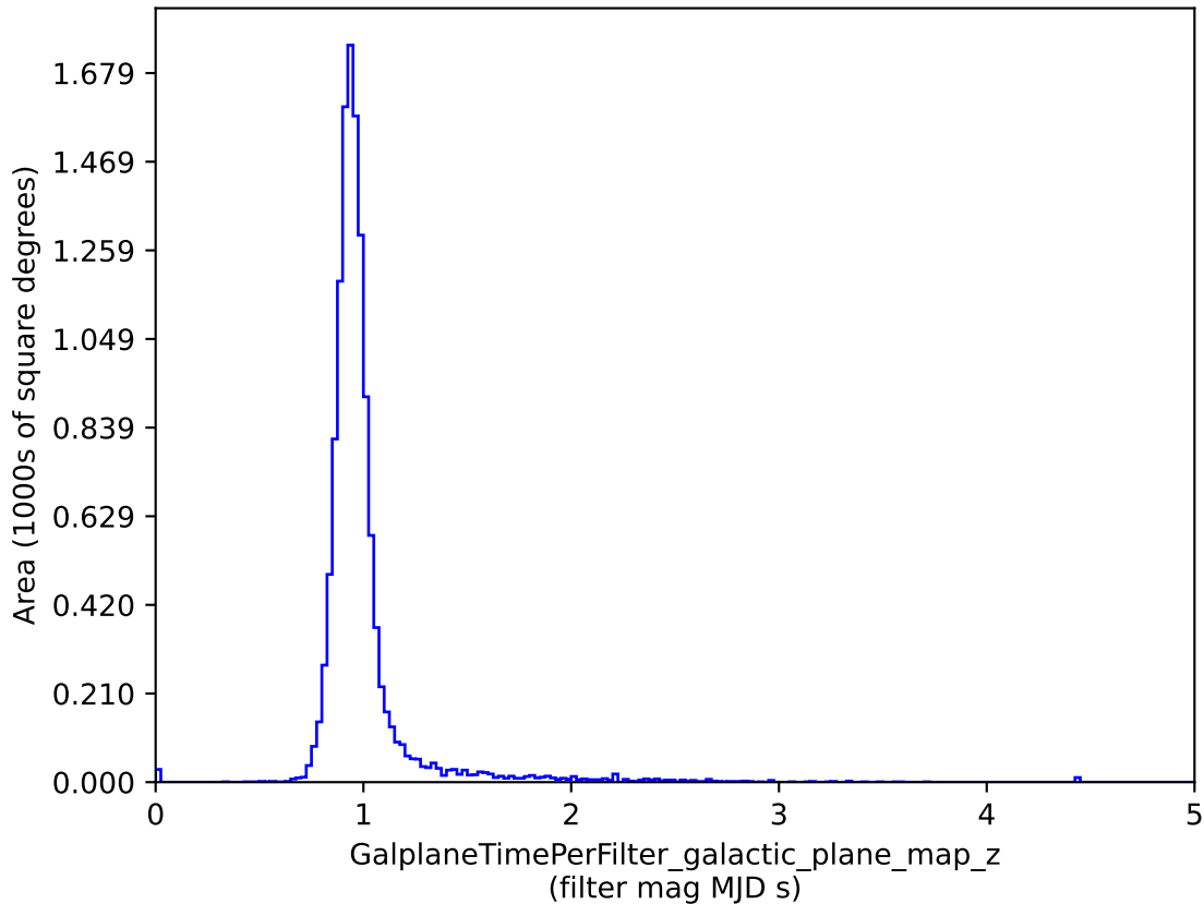
baseline_v3.4_10yrs : GalplaneTimePerFilter_galactic_plane_map_z
