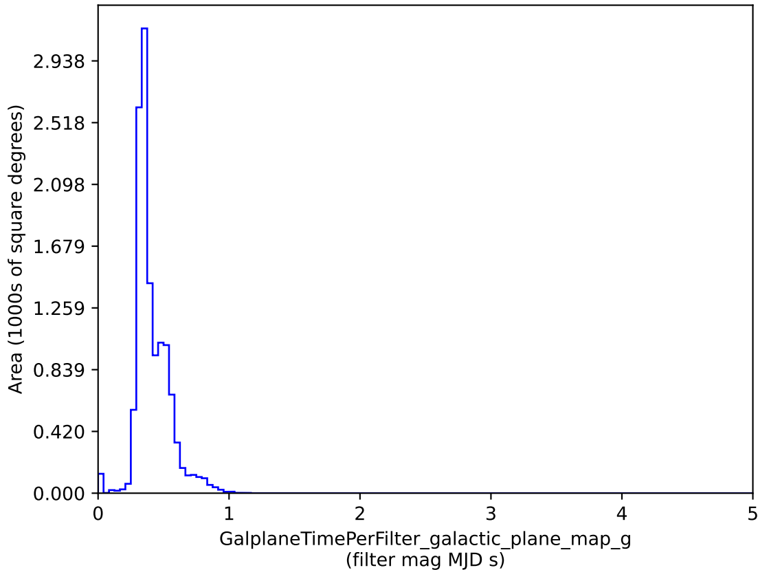
baseline_v3.4_10yrs : GalplaneTimePerFilter_galactic_plane_map_g
