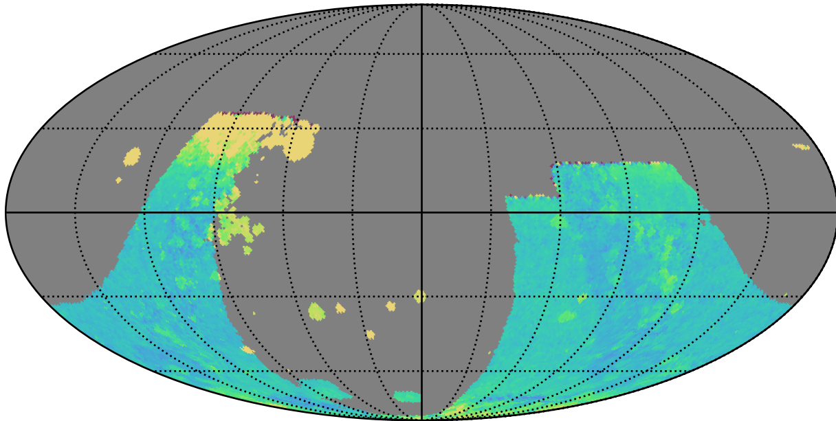
baseline_v3.4_10yrs : GalplaneTimePerFilter_combined_map_z
