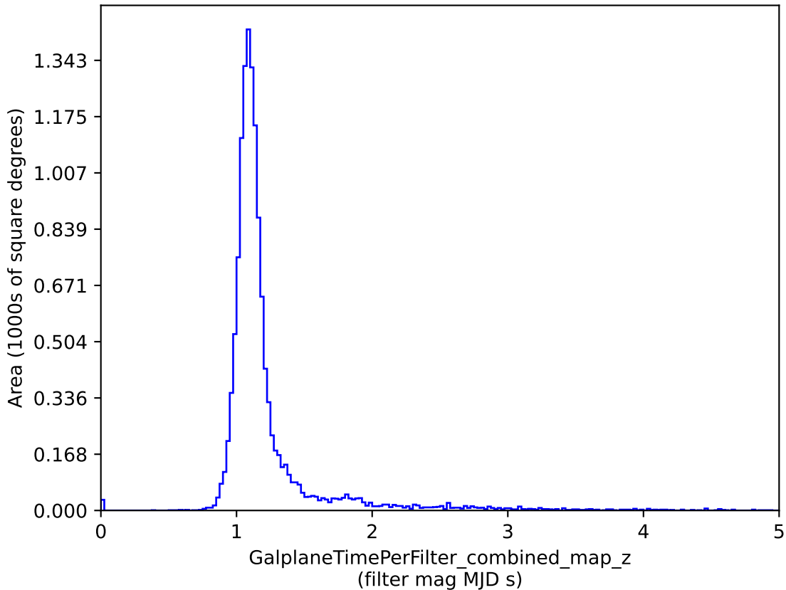
baseline_v3.4_10yrs : GalplaneTimePerFilter_combined_map_z
