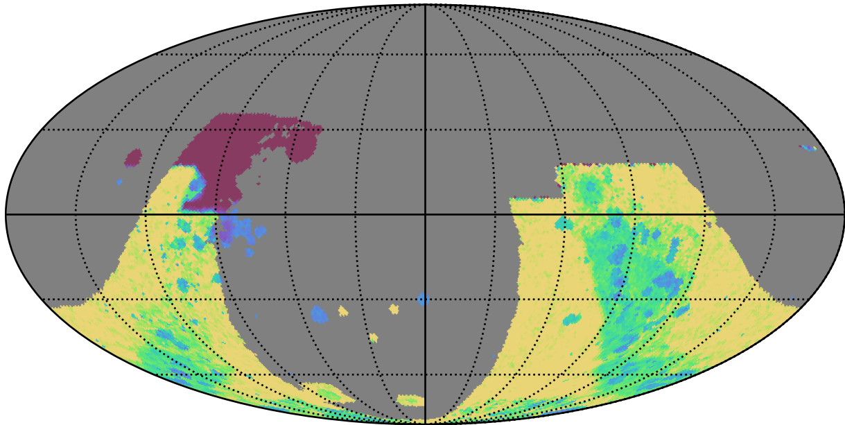
baseline_v3.4_10yrs : GalplaneTimePerFilter_combined_map_y
