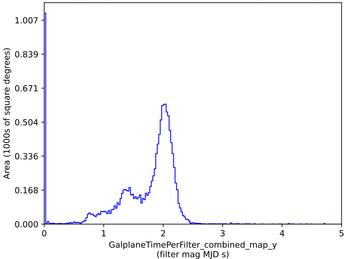
baseline_v3.4_10yrs : GalplaneTimePerFilter_combined_map_y
