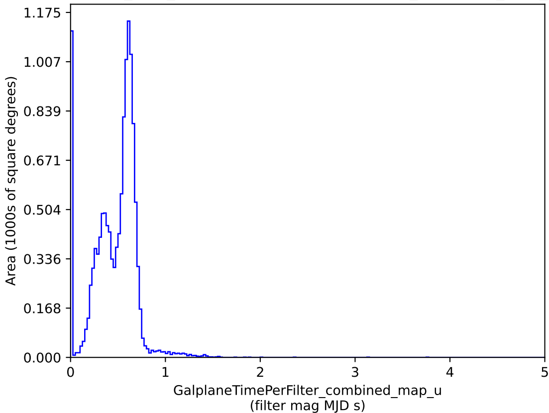
baseline_v3.4_10yrs : GalplaneTimePerFilter_combined_map_u
