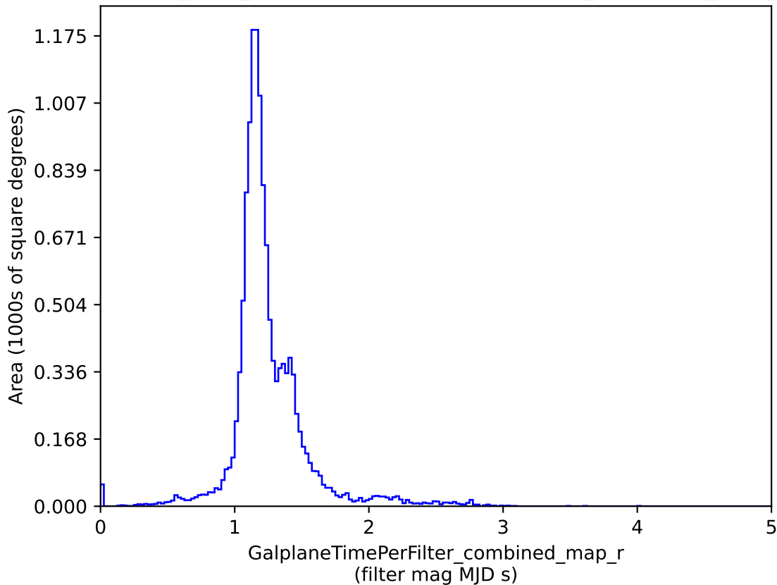
baseline_v3.4_10yrs : GalplaneTimePerFilter_combined_map_r
