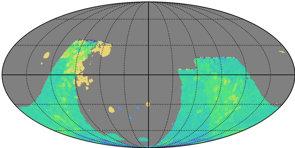
baseline_v3.4_10yrs : GalplaneTimePerFilter_combined_map_i
