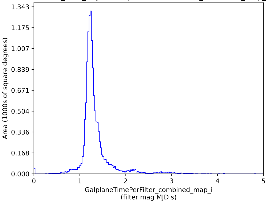
baseline_v3.4_10yrs : GalplaneTimePerFilter_combined_map_i
