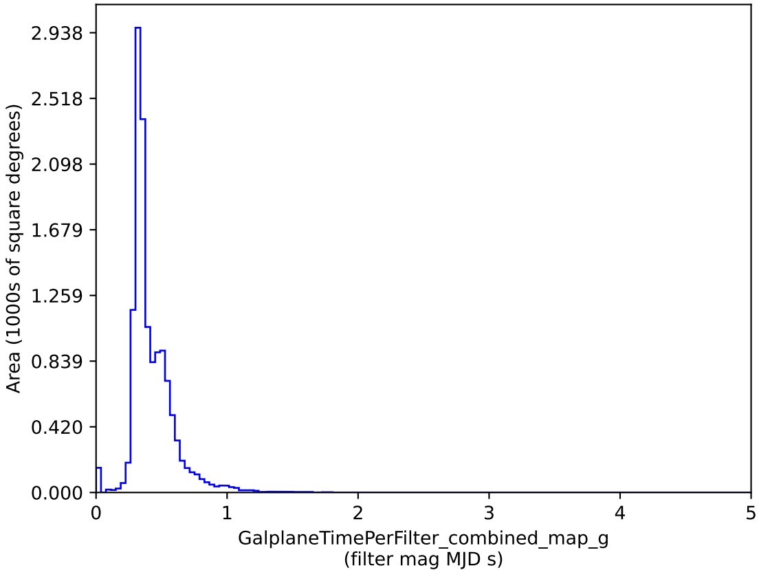
baseline_v3.4_10yrs : GalplaneTimePerFilter_combined_map_g
