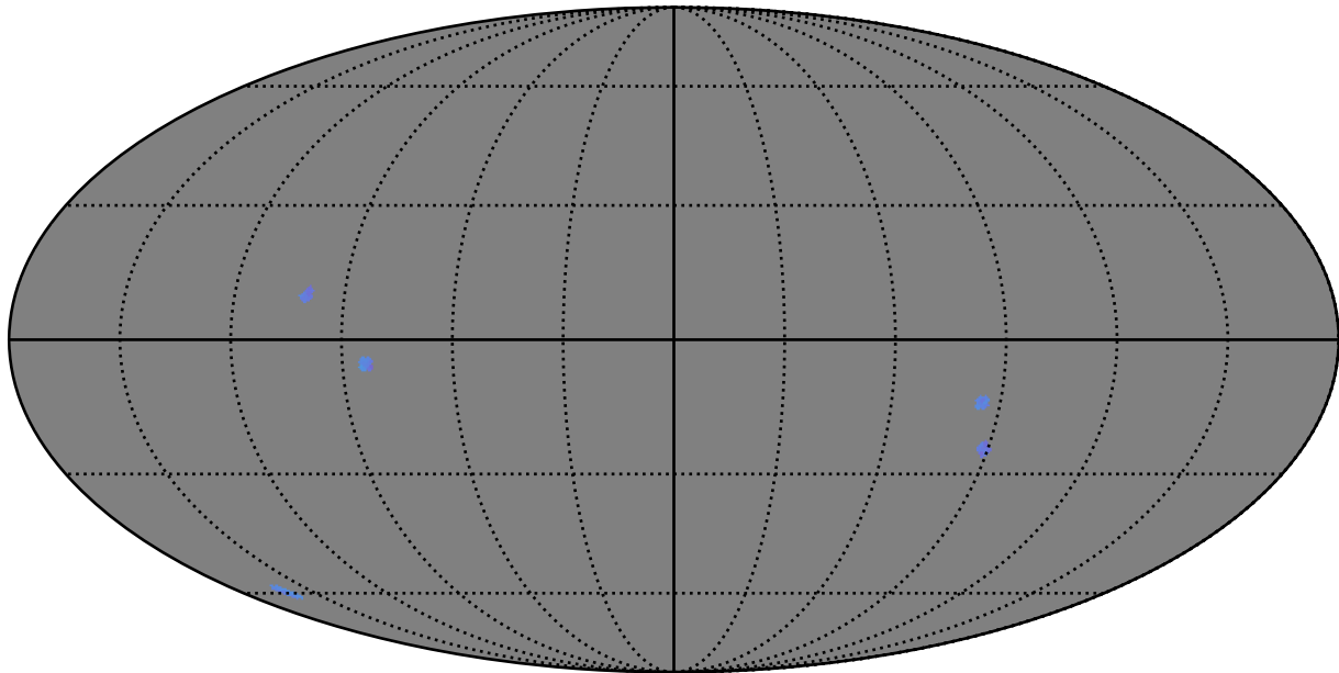
baseline_v3.4_10yrs : GalplaneTimePerFilter_bonito_sfr_map_g
