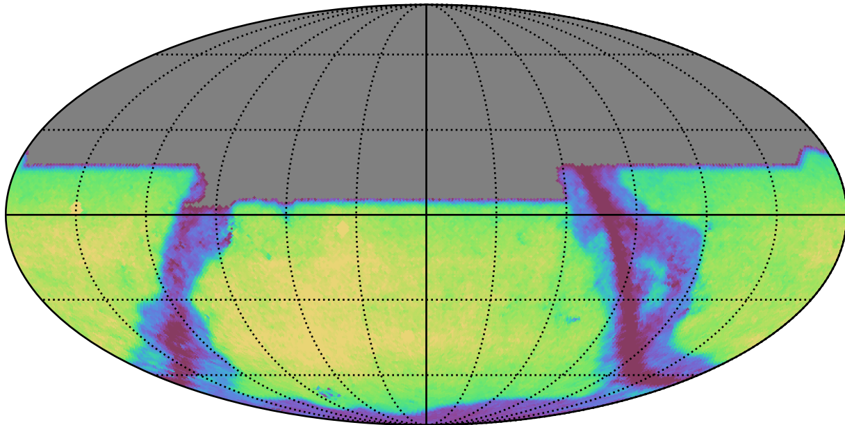
baseline_v3.4_10yrs y: GalaxyCountsMetricExtended
