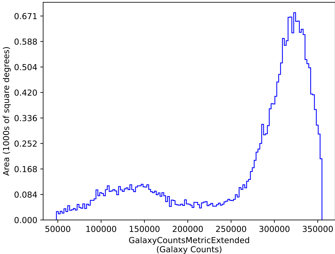
baseline_v3.4_10yrs y: GalaxyCountsMetricExtended
