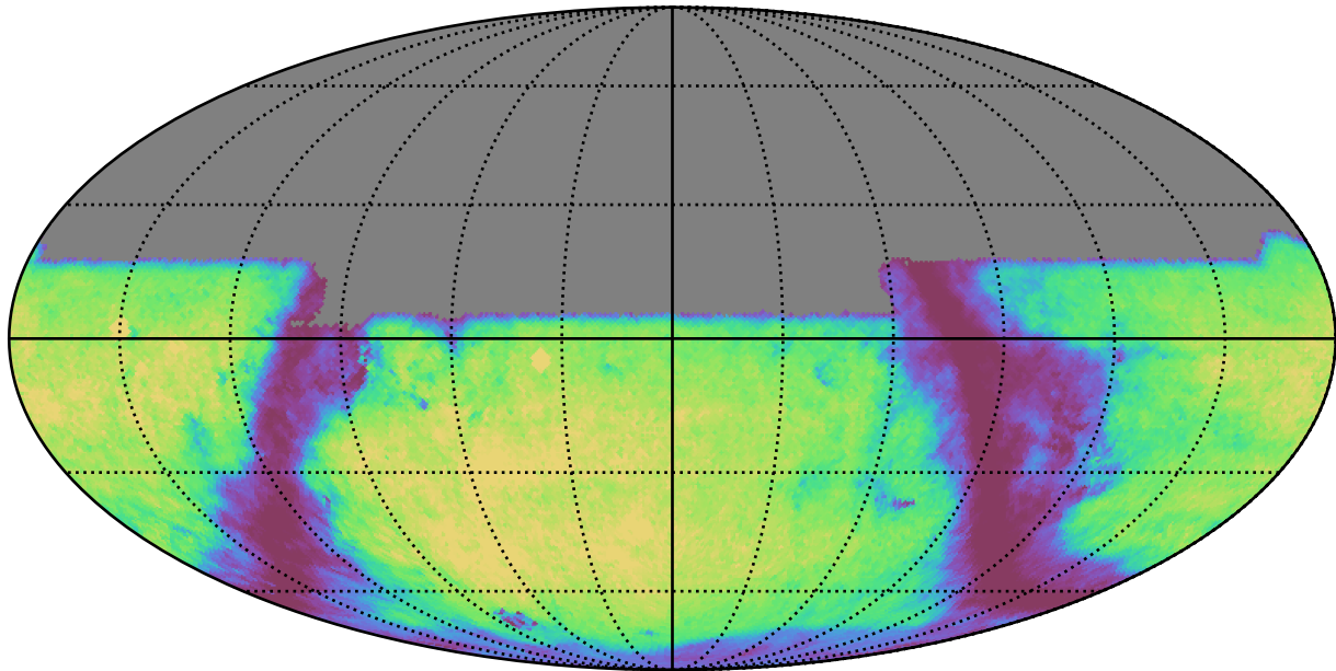
baseline_v3.4_10yrs u: GalaxyCountsMetricExtended
