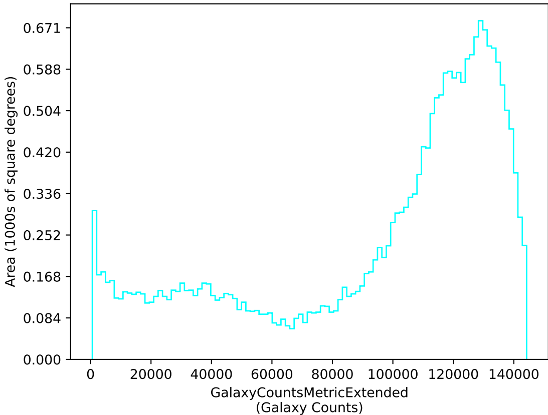
baseline_v3.4_10yrs u: GalaxyCountsMetricExtended
