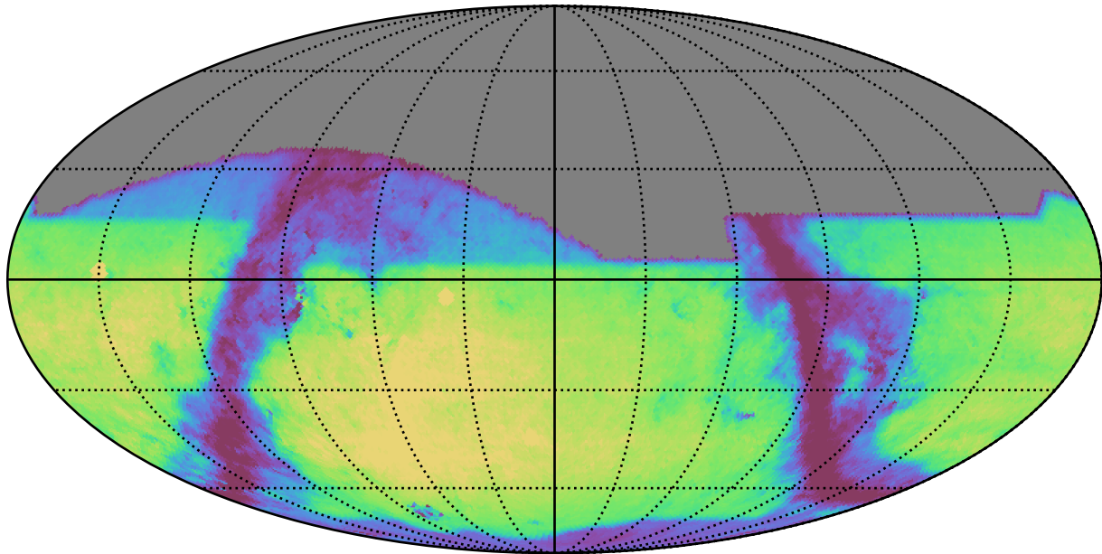
baseline_v3.4_10yrs r: GalaxyCountsMetricExtended
