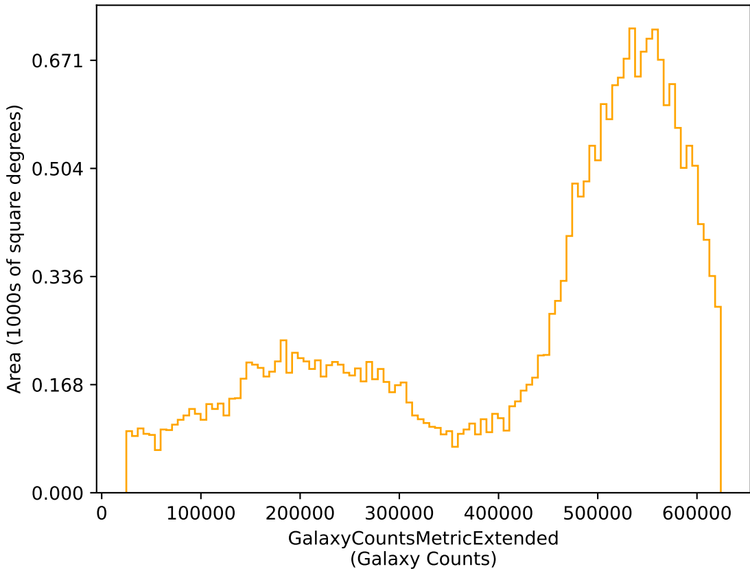
baseline_v3.4_10yrs r: GalaxyCountsMetricExtended
