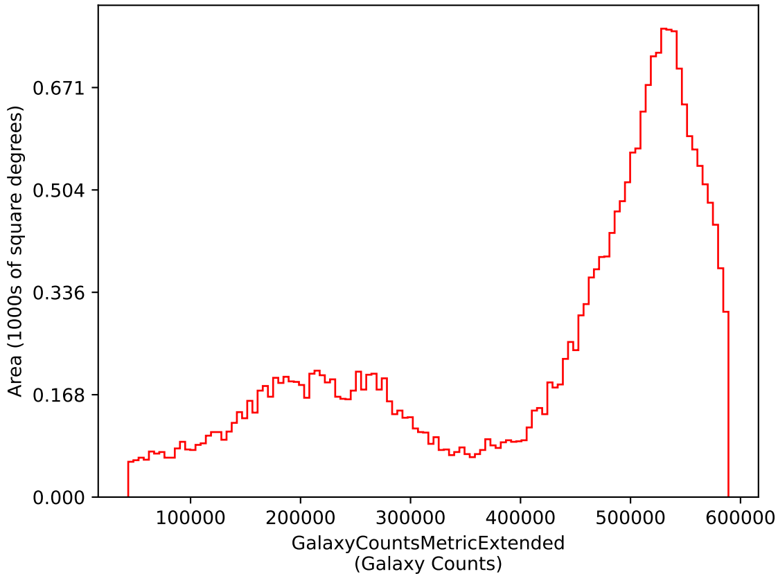
baseline_v3.4_10yrs i: GalaxyCountsMetricExtended
