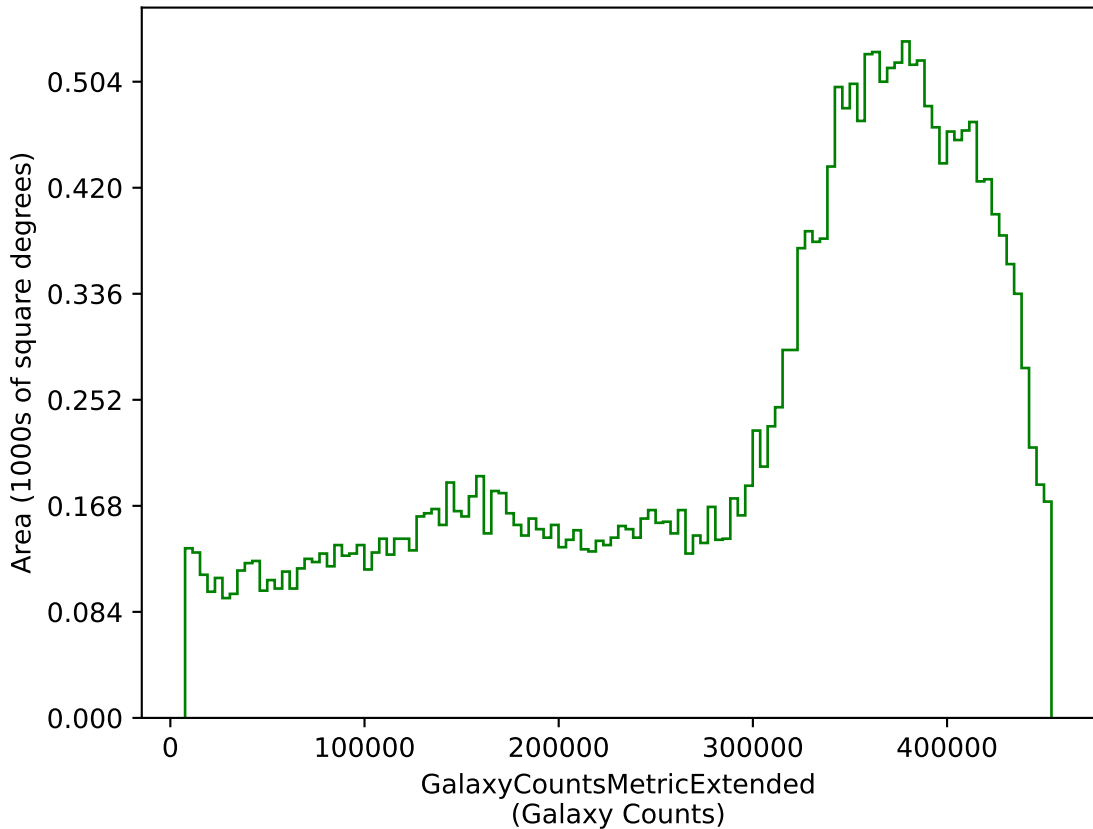
baseline_v3.4_10yrs g: GalaxyCountsMetricExtended
