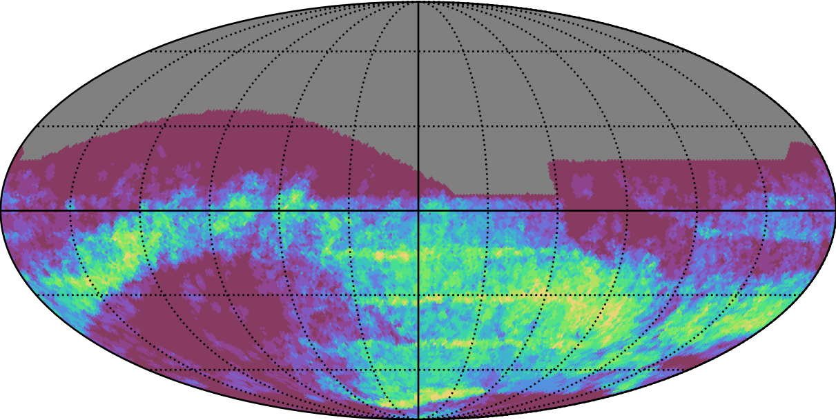
baseline_v3.4_10yrs : GalPlaneSeasonGapsTimescales_xray_binaries_map_Tau_10_0
