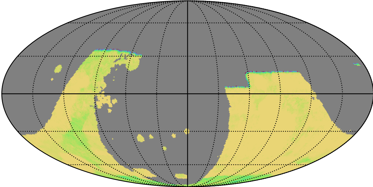
baseline_v3.4_10yrs : GalPlaneSeasonGapsTimescales_combined_map_Tau_232_5
