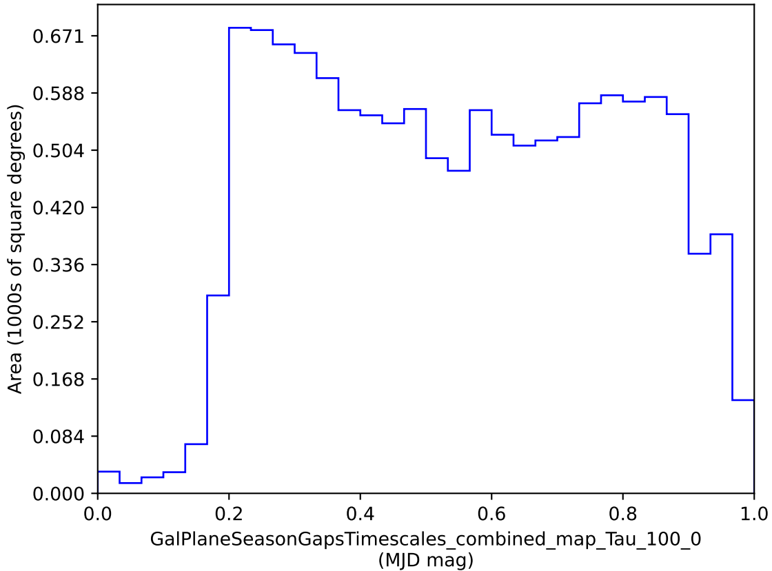
baseline_v3.4_10yrs : GalPlaneSeasonGapsTimescales_combined_map_Tau_100_0
