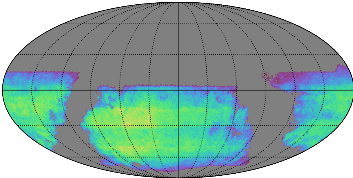
baseline_v3.4_10yrs i band non-DD year 9: ExgalM5WithCuts
