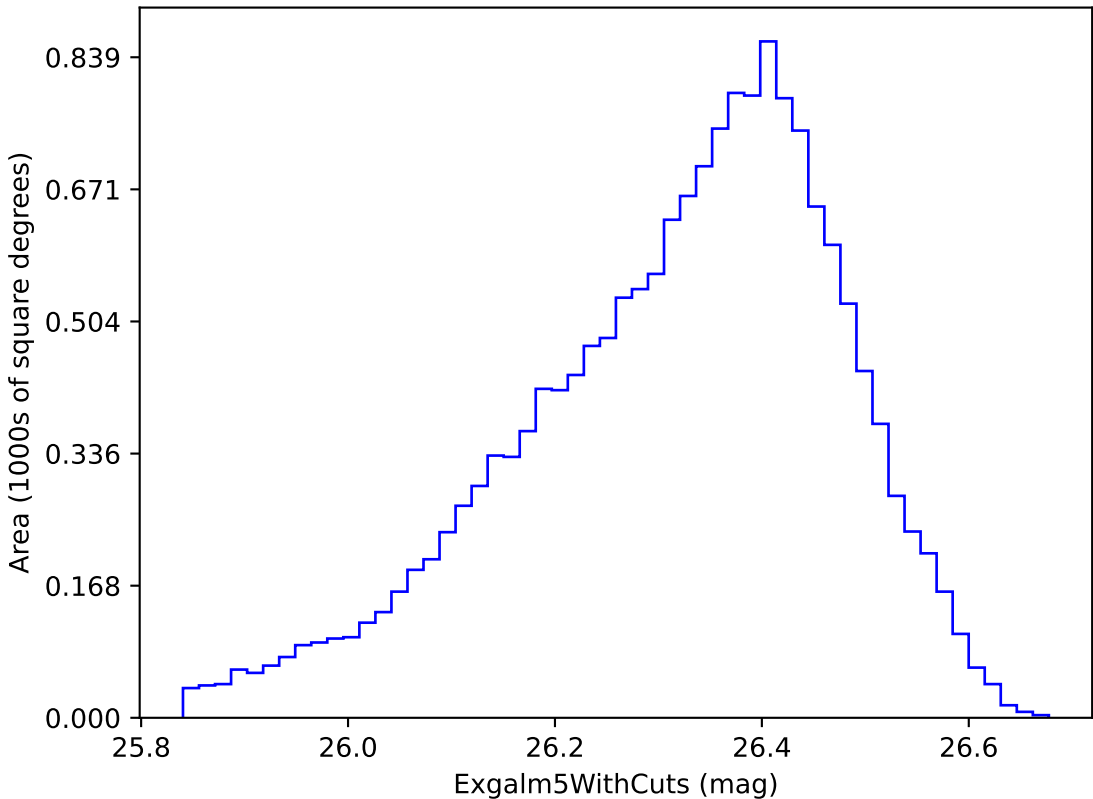
baseline_v3.4_10yrs i band non-DD year 9: ExgalM5WithCuts
