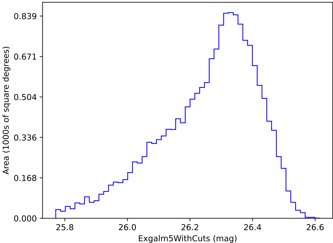
baseline_v3.4_10yrs i band non-DD year 8: ExgalM5WithCuts
