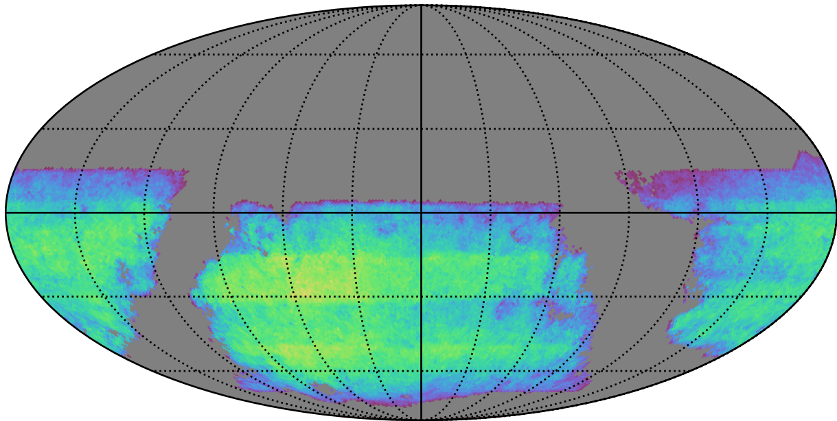
baseline_v3.4_10yrs i band non-DD year 7: ExgalM5WithCuts
