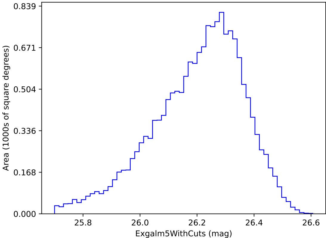
baseline_v3.4_10yrs i band non-DD year 7: ExgalM5WithCuts
