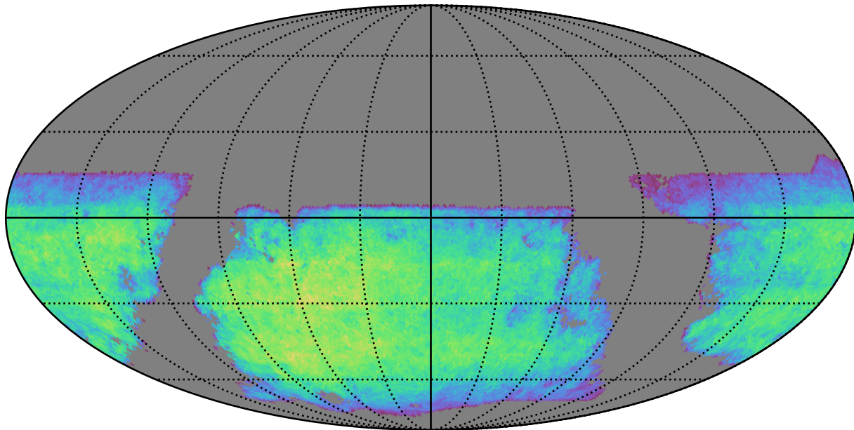
baseline_v3.4_10yrs i band non-DD year 6: ExgalM5WithCuts
