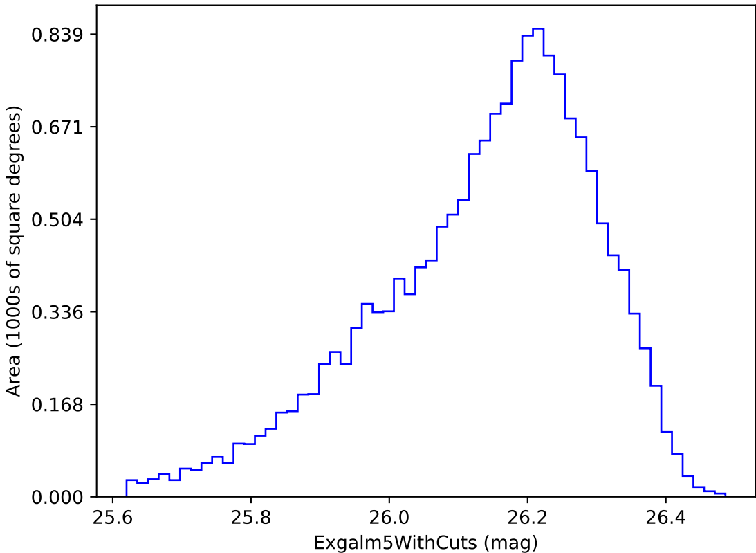
baseline_v3.4_10yrs i band non-DD year 6: ExgalM5WithCuts
