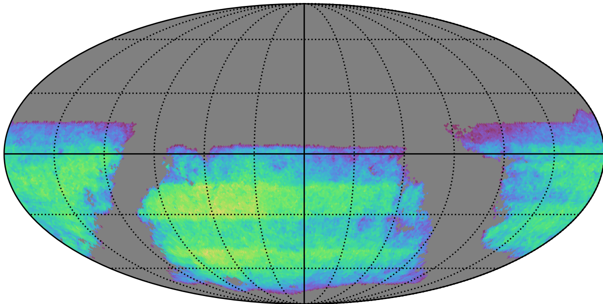
baseline_v3.4_10yrs i band non-DD year 5: ExgalM5WithCuts
