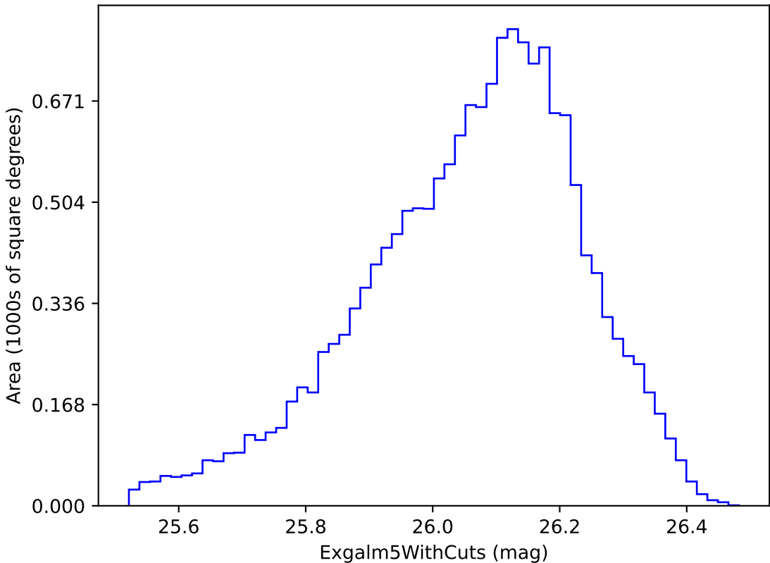
baseline_v3.4_10yrs i band non-DD year 5: ExgalM5WithCuts
