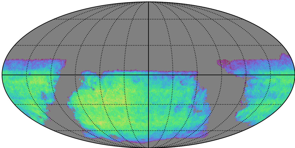
baseline_v3.4_10yrs i band non-DD year 4: ExgalM5WithCuts
