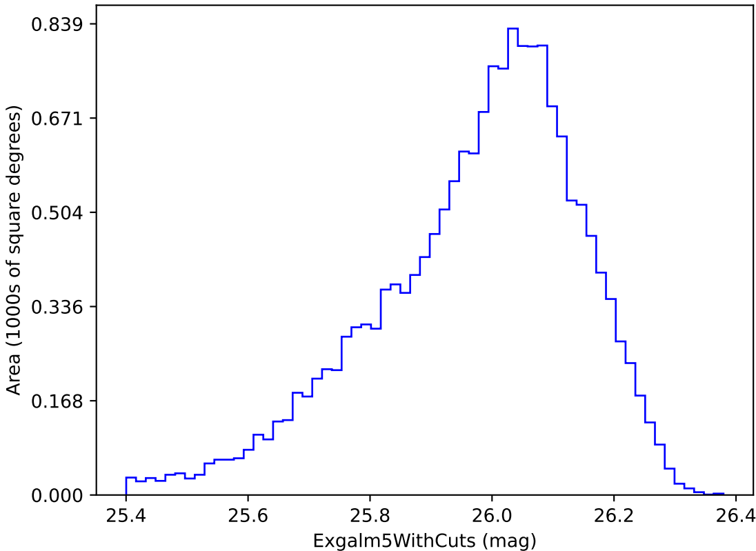
baseline_v3.4_10yrs i band non-DD year 4: ExgalM5WithCuts
